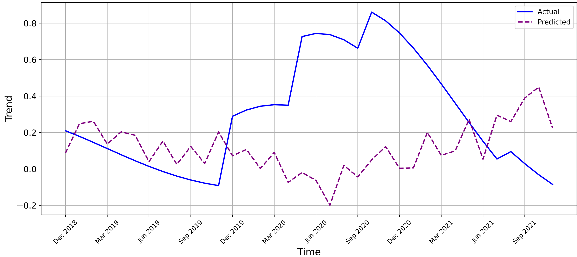
Solution_SPATIAL SMOOTHING_Mentions - Validation
